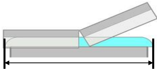
For spa cabinets with no rail: Measure from the widest point on the acrylic lip.
