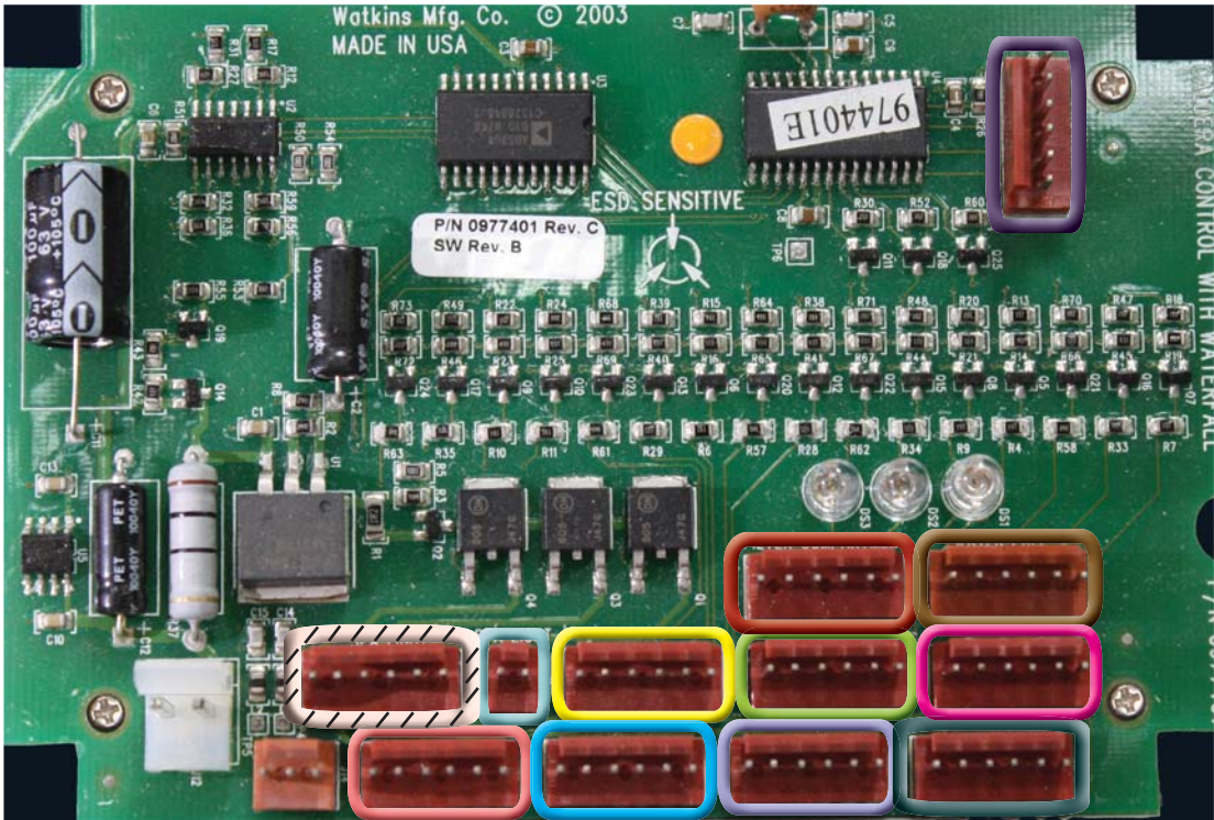
SpaGlo ® MODULE (FACTORY INSTALLED)
