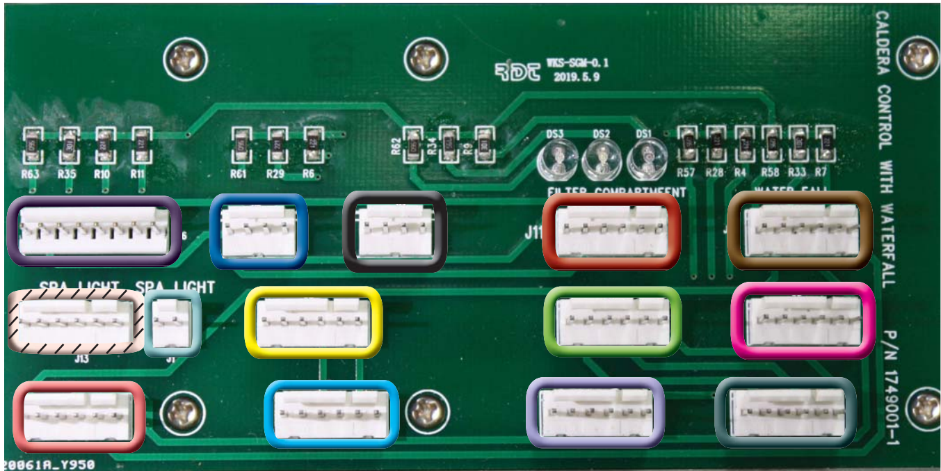
SpaGlo ® CONTROLLER EAGLE RETROFIT
