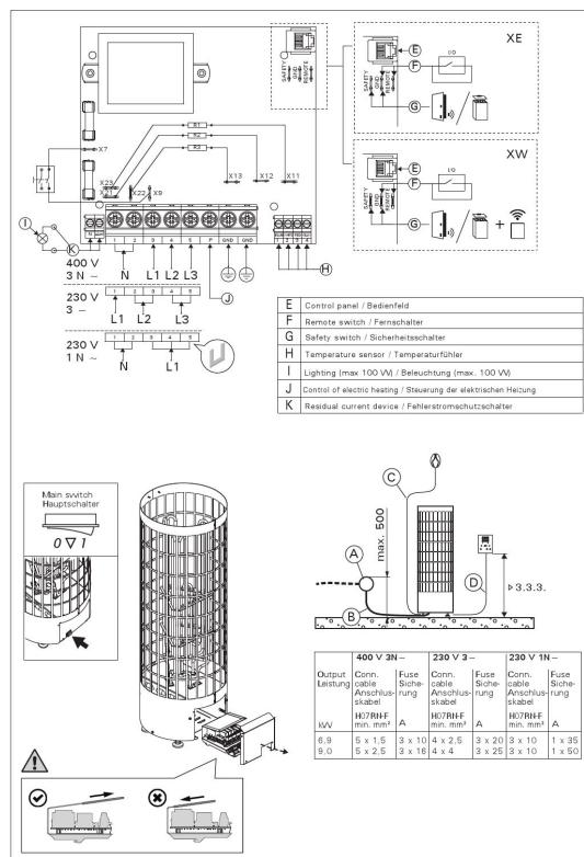
Electrical connections
