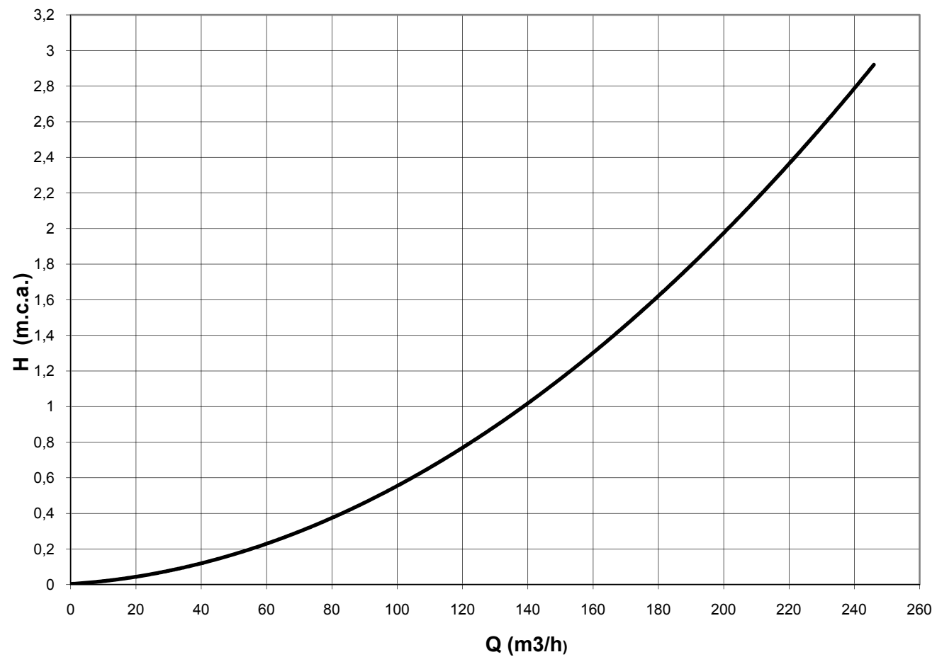
Prefiltro Aral 37 I Aral 37 I pre-filter
