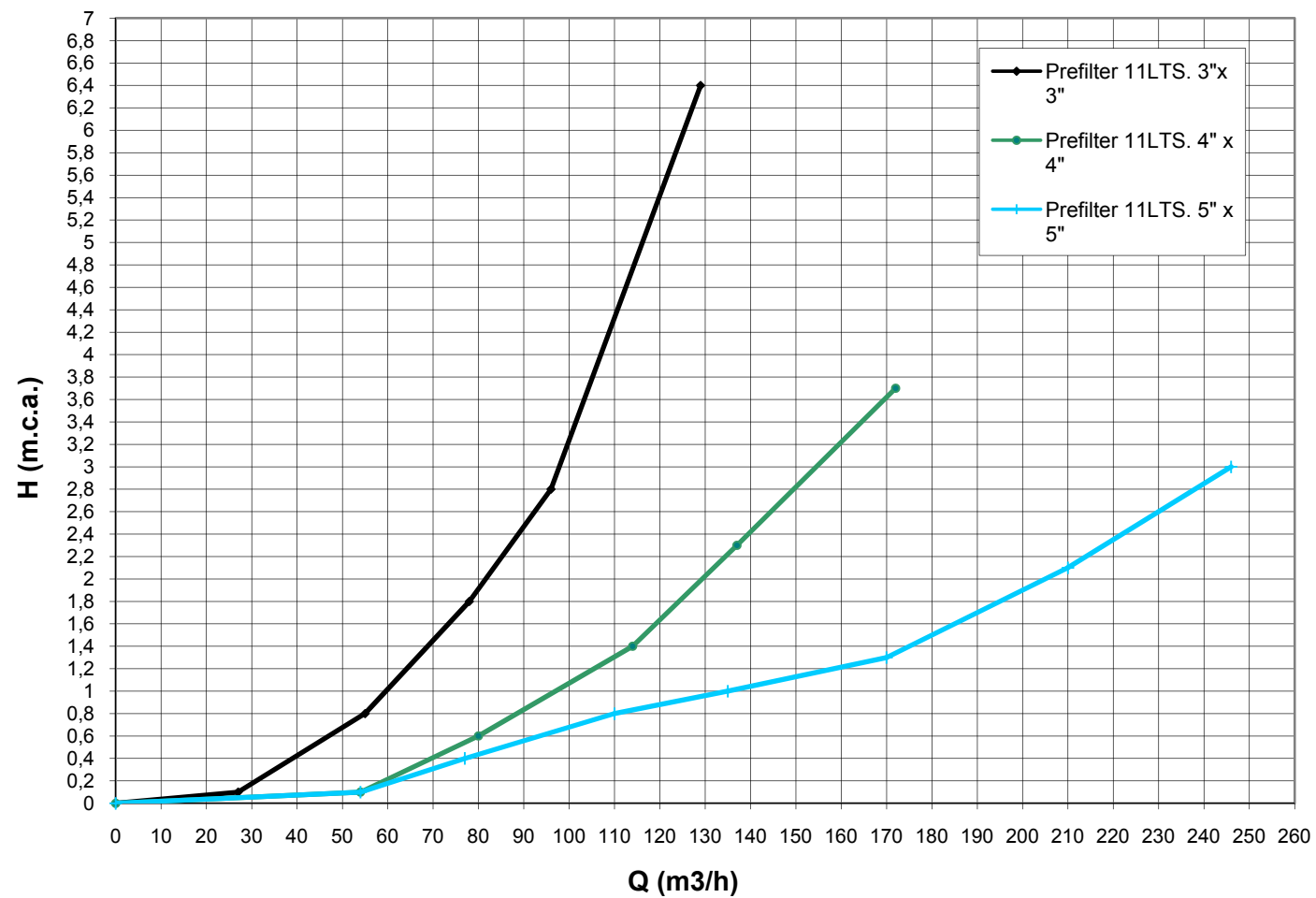
Prefiltro Aral 11 I Aral 11 I pre-filter
