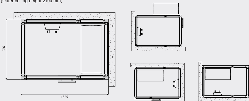
Tylö steam shower i170 (Outer ceiling height 2100 mm)
